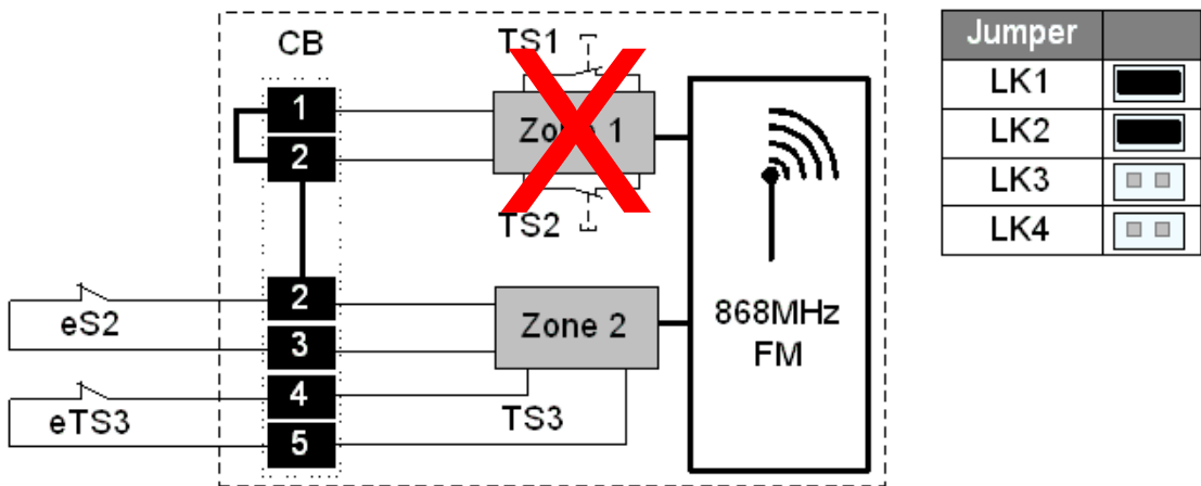
Fig.8 Zone 2 - 1 x NC / eS2 + 1 NC / eTS
