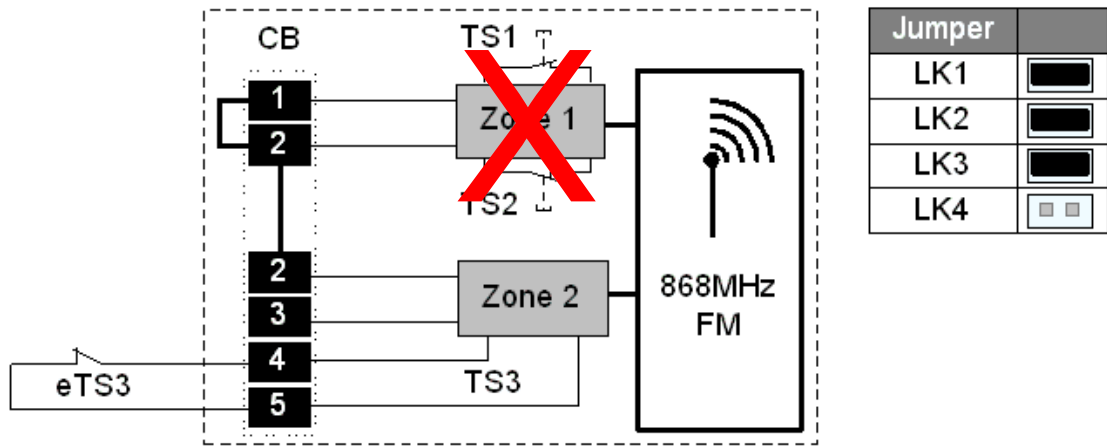
Fig.6 Zone 2 - 1 x NC / eTS3
