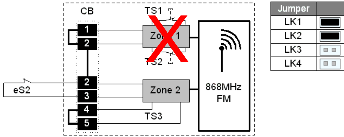
Fig.4 Zone 2 - 1 x NC / eS2
