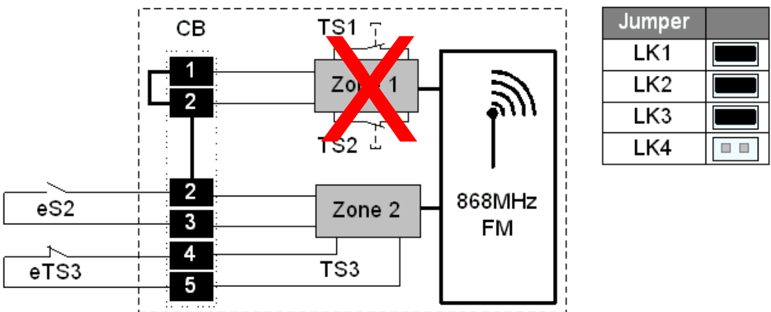
Fig.7 Zone 2 - 1 x NO / eS2 + 1 NC / eTS
