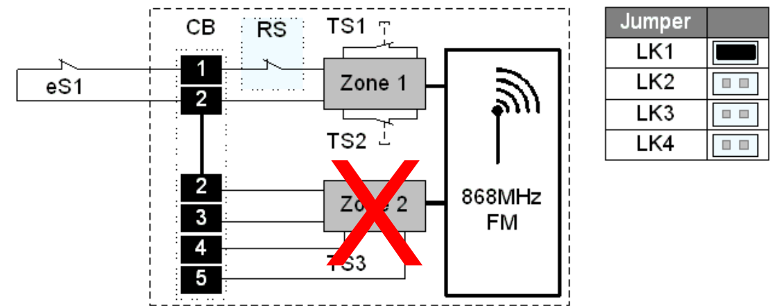
Fig.2 Zone 1 - 1 x NC / RS + 1 x NC / eS1
