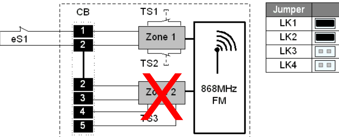
Fig.3 Zone 1 - 1 x NC / eS1
