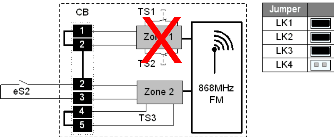
Fig.5 Zone 2 - 1 x NO / eS2
